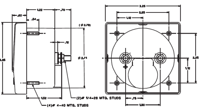
VISTA 312 Analog Panel Meter Size 3½"
