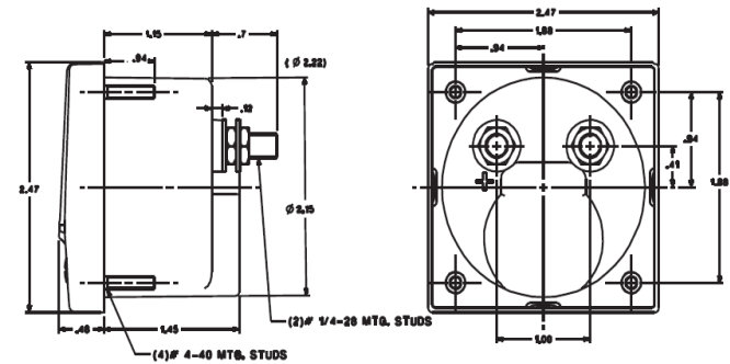
VISTA 312 Analog Panel Meter Size 3½"
