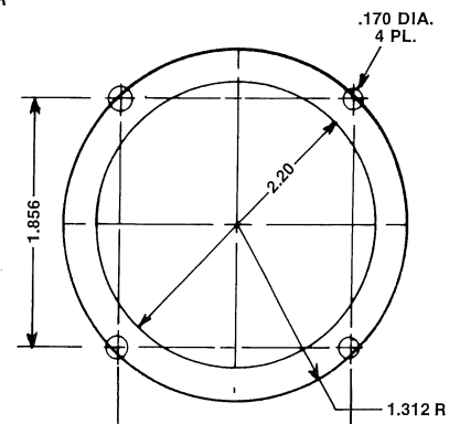
PANEL DRILLING PLAN
