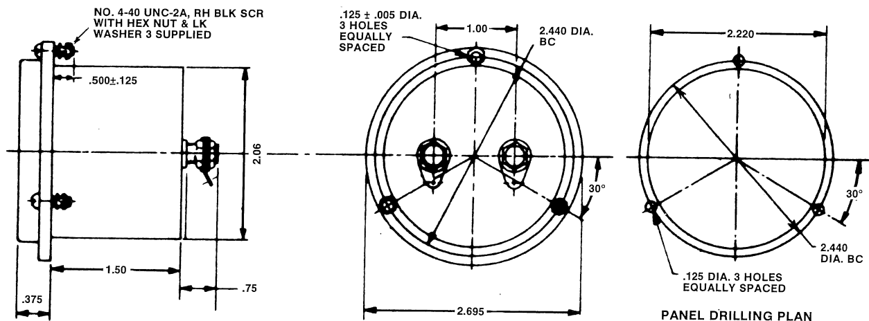
2 1/2" MODEL 266
