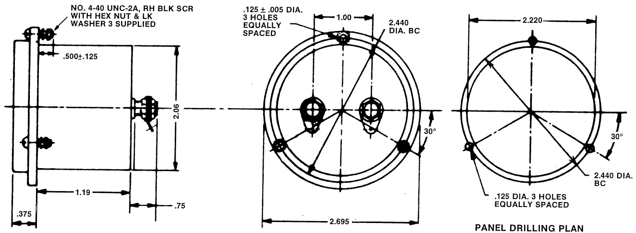
2 1/2" MODEL 266
