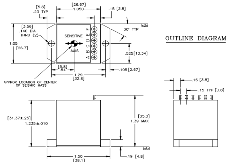
Outline Drawing: Dimensional Drawing for the LSM Accelerometer (inch/mm)
